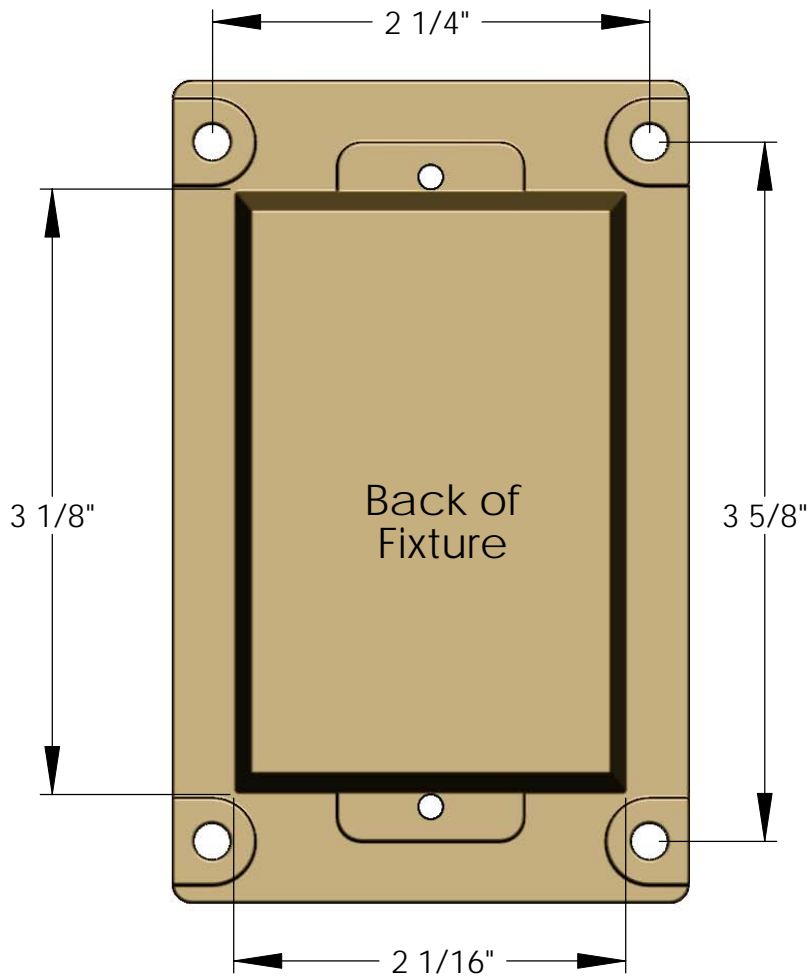
Back of Fixture Drilling Template for 1542BZ Full Scale
