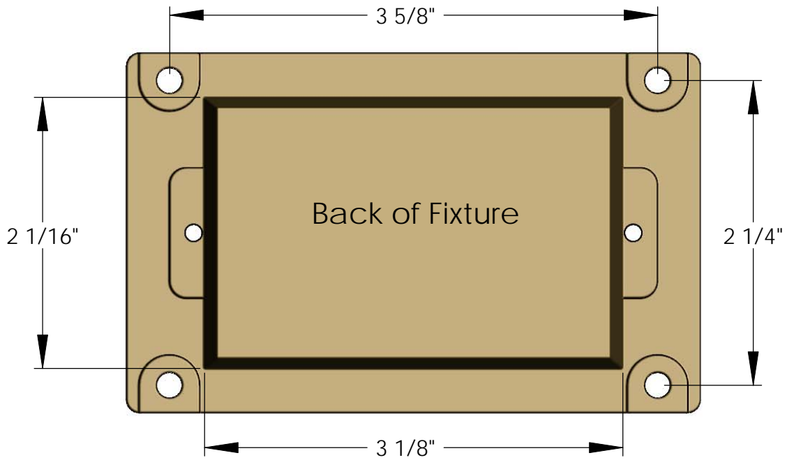
Back of Fixture Drilling Template for 1546BZ Full Scale
